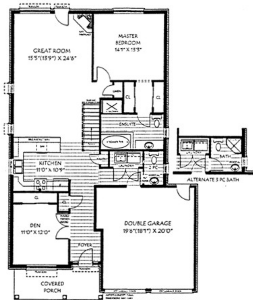
THE BIRMINGHAM 1,420 SQFT
