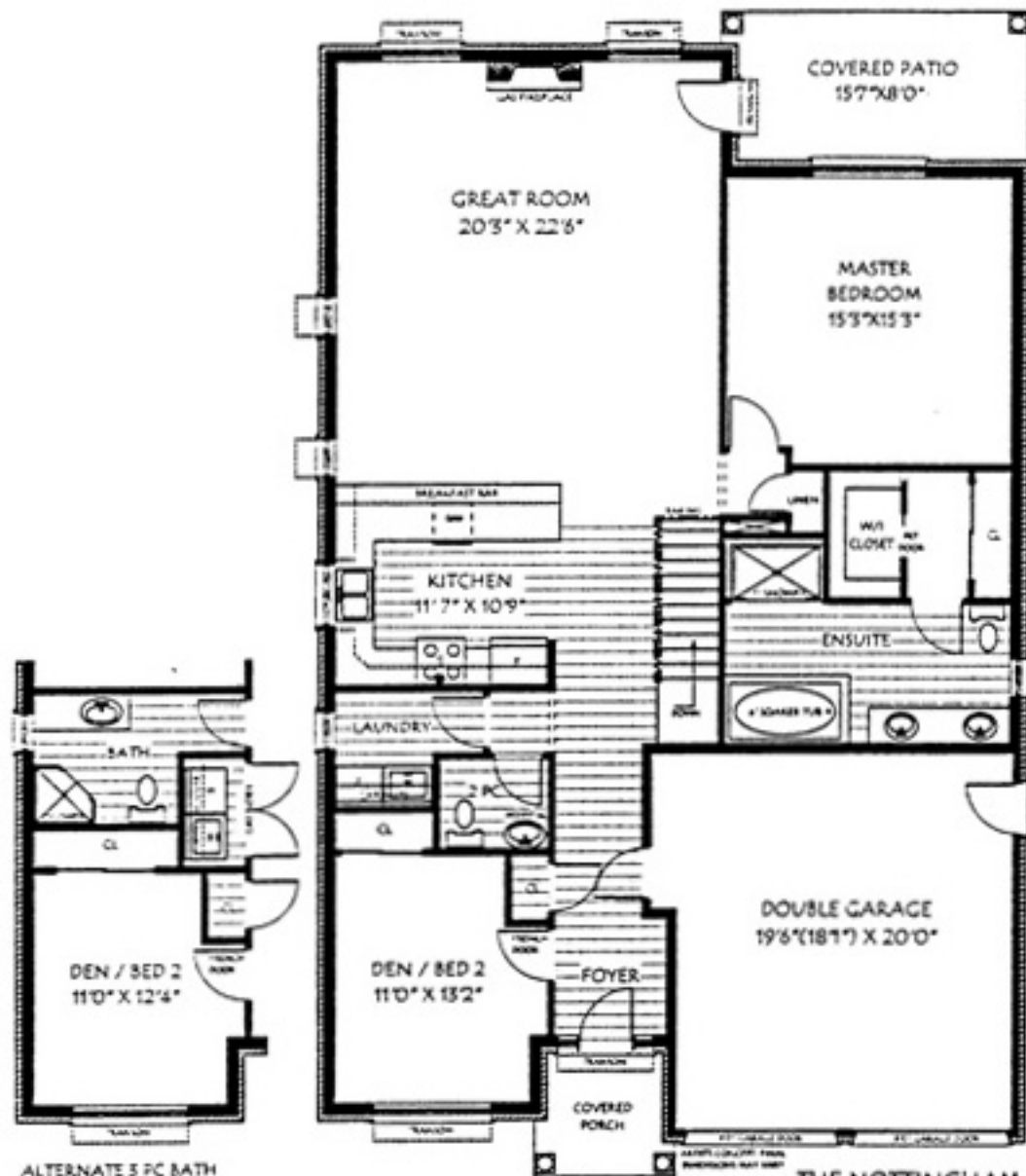
THE NOTTINGHAM 1,650 SQFT
